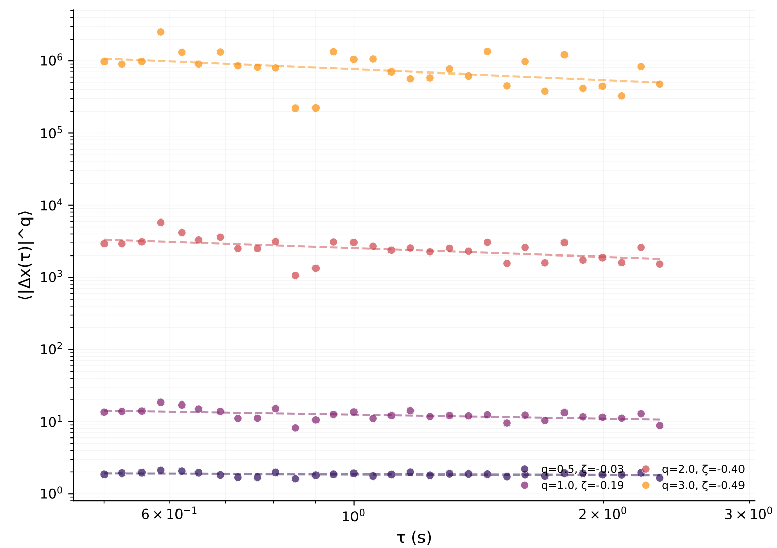
S-wave
