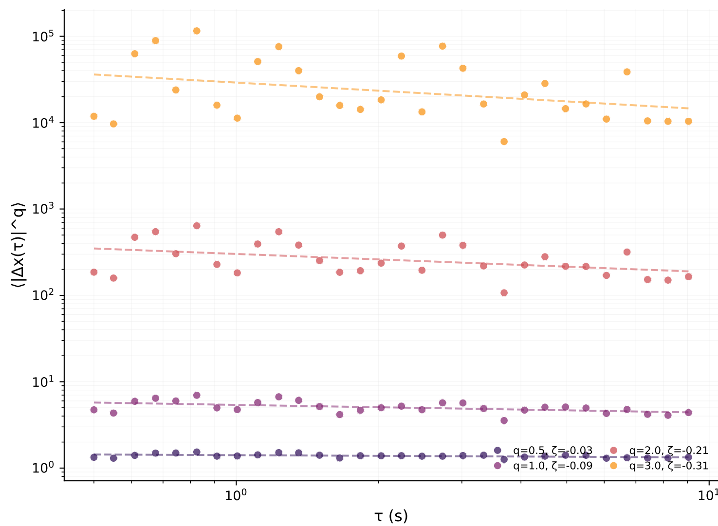
Coda
