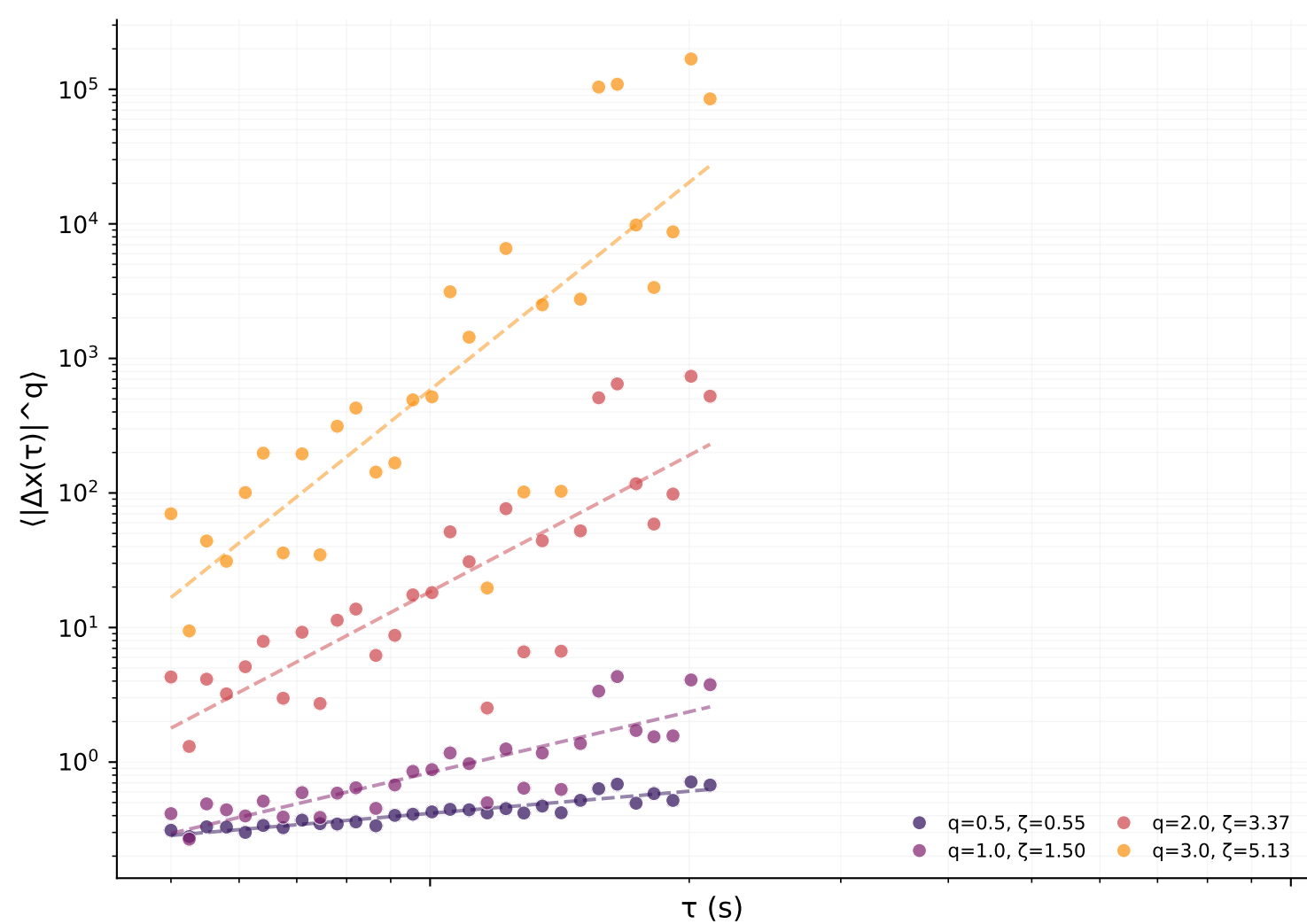
Coda
